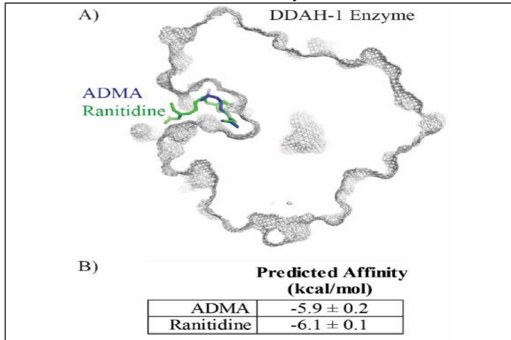
3 Figure 2 – Computational Modelling of Ranitidine Binding to 4 DDAH-1 Enzyme
