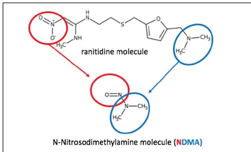
14 Figure 1 – Ranitidine Structure & Formation of NDMA
