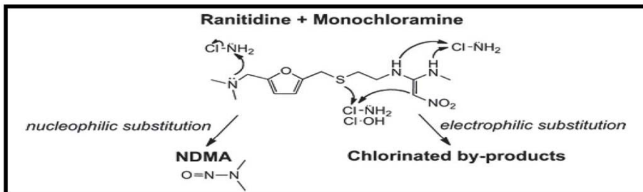
Figure 2 – Mechanism for Decomposition of Ranitidine in NDMA
